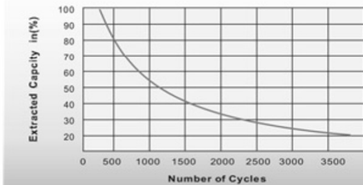
Cycle Service Life
